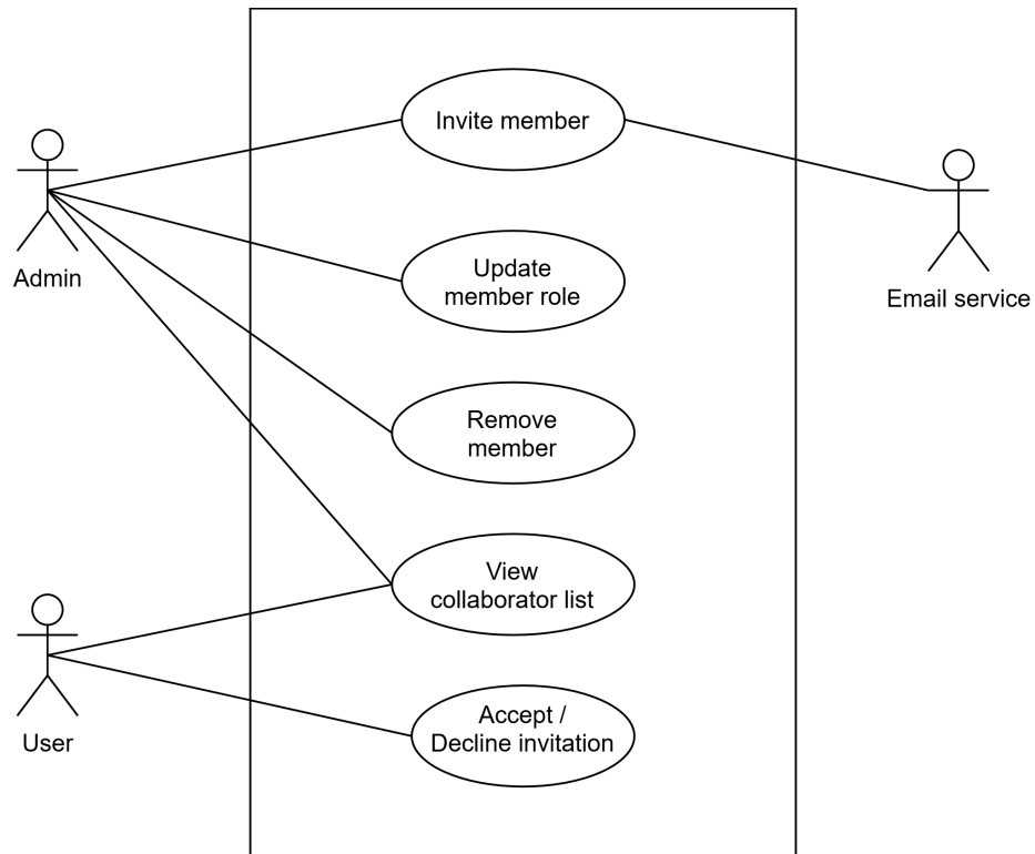
Figure 9: Use case diagram — Level 1.7: Team Collaboration
